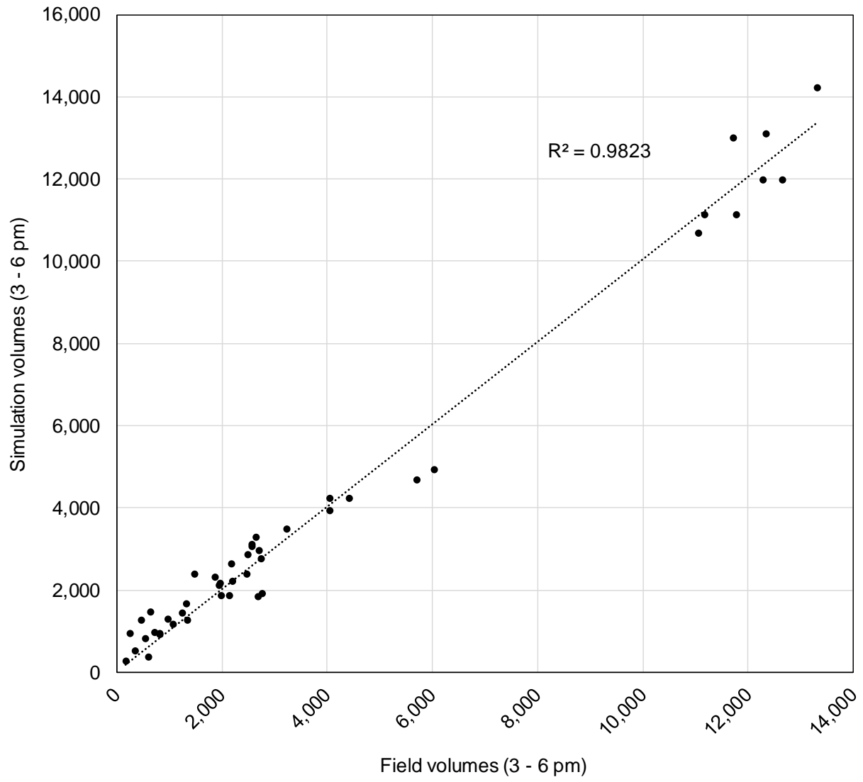
Figure 3: Layton VISUM Network Calibration
